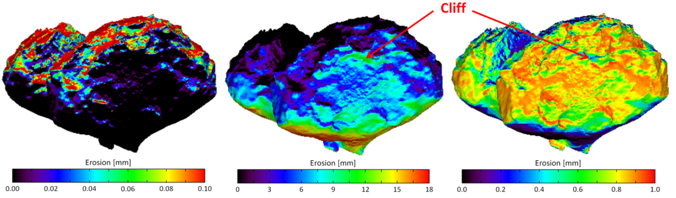
Fig. 17. Erosion per spin (model B) on the large Imhotep plain when the sub-solar latitude is 48° ( left image , May 2014), at southern solstice ( center image , September 2015), and at equinox ( right image , March 2016). The view is in the equatorial plane. The rotation axis is inclined by about 50° relative to the Imhotep plain. At southern solstice the cliff (indicated) is insulated and eroded much stronger than at equinox, when the Sun is high but farther away.
