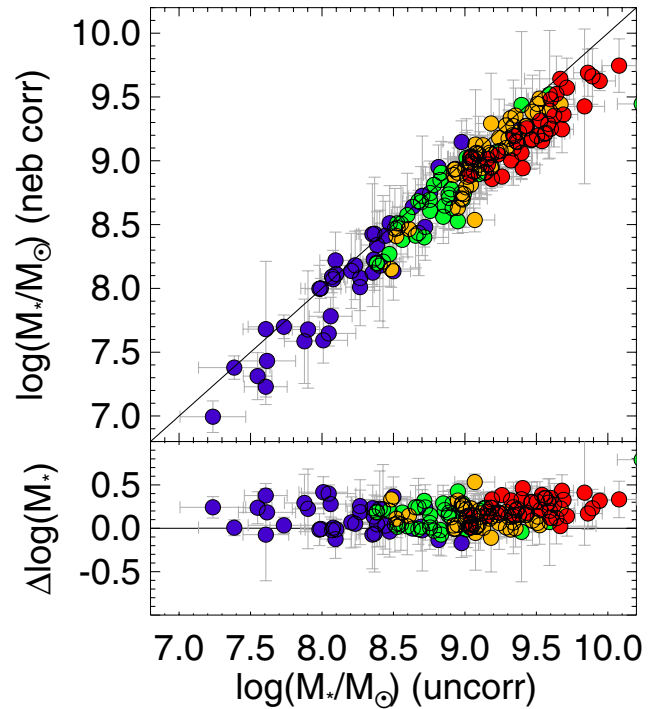
Fig. 6. Comparison of stellar masses derived from SED fitting before (uncorr, x -axis) and after (nebcorr, y -axis) removing the contribution of emission line fluxes to the broadband photometry. Bottom panel: difference in stellar mass (uncorr–nebcorr) on the y -axis. Symbols and colors are as in Fig. 3.
