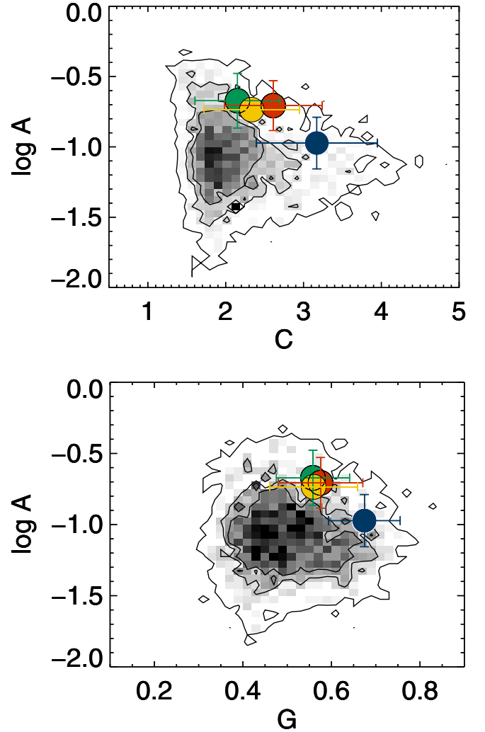
Fig. 13. Asymmetry-concentration (top) and asymmetry-Gini (bottom) diagrams. The gray density plot shows the location of the SFG-20k sample. The inner and outer contours enclose 50, 68 and 95% of the sample, respectively. Median values and dispersions for the EELGs are indicated by large color circles and error bars. Yellow, red, green and blue colors indicate EELGs visually classified as “merger/interaction”, “cometary/tadpole”, “clumpy/chain” and “round/nucleated”, respectively.
