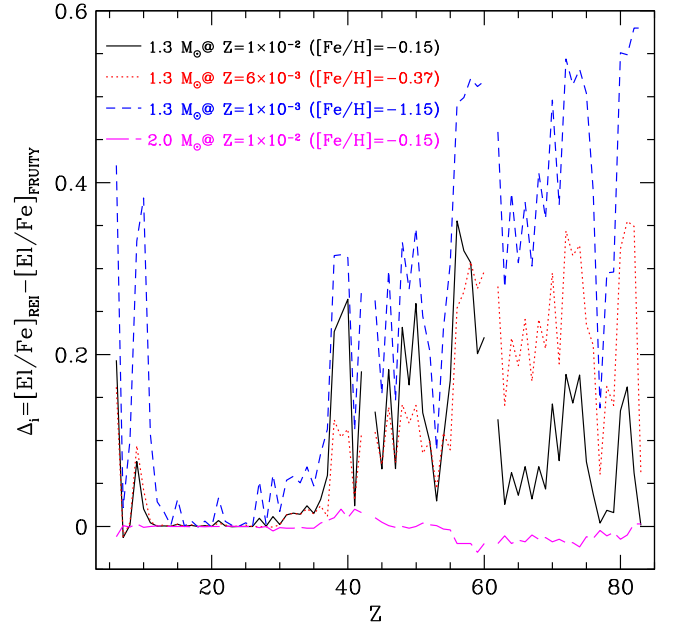
Figure 10. Differences in the surface chemical distributions of 1.3 M_{\odot} stars at various metallicities computed with a different RGB mass-loss rate (REI: \eta_R = 0.2 ) with respect to the corresponding FRUITY models (FRUITY: \eta_R = 0.4 ). A 2.0 M_{\odot} star is also reported for comparison.
