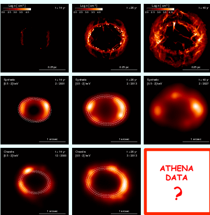
Fig. 2. Interaction of the blast wave with the nebula.
