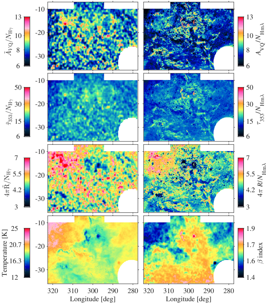
Fig. 11. Three upper rows: spatial variations of the dust properties per gas nucleon with the total gas measured by N_{\text{H}\gamma} on a 0'.375 pixel grid (left) and by N_{\text{H}m,l} on a 0'.125 pixel grid (right). Lower row: colour temperature and \beta index of the dust SED, measured at 5' resolution by Planck Collaboration XI (2014) and displayed on a 0'.125 pixel grid. The A_{VQ}/N_H values are in units of 10^{-22} mag \text{cm}^2 , \tau_{353}/N_H in 10^{-27} \text{cm}^2 , and 4\pi R/N_H in 10^{-31} W.
