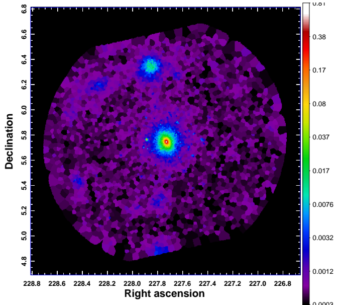
Figure 4. ROSAT /SPC surface-brightness image of A2029 obtained using Voronoi tessellation (Cappellari & Copin 2003), in units of \text{cts s}^{-1} \text{ arcmin}^{-2} . Each Voronoi bin includes an average of 20 counts.
