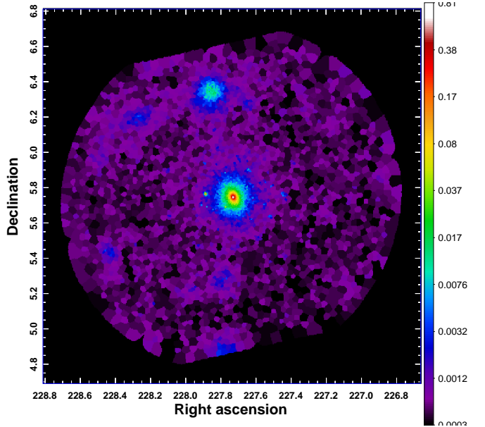
Figure 4. ROSAT/PSPC surface-brightness image of A2029 obtained using Voronoi tessellation (Cappellari & Copin 2003), in units of \text{cts s}^{-1} \text{ arcmin}^{-2} . Each Voronoi bin includes an average of 20 counts.
