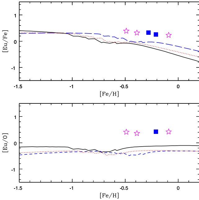
Figure 11. In these figures, we compare the predictions of our models with different IMFs for the [Eu/Fe] and [Eu/O] versus [Fe/H] abundance patterns, when the yield of Cescutti et al. (2006) are included. The latter assume the Eu to be produced by massive stars with mass in the range M = 12\text{--}30 M_{\odot} , which explode as core-collapse SNe. None of the models with these yields is able to reproduce both the [Eu/Fe] and [Eu/O] abundance ratio patterns at the same time. The various lines correspond to the same IMFs as in Fig. 3.
