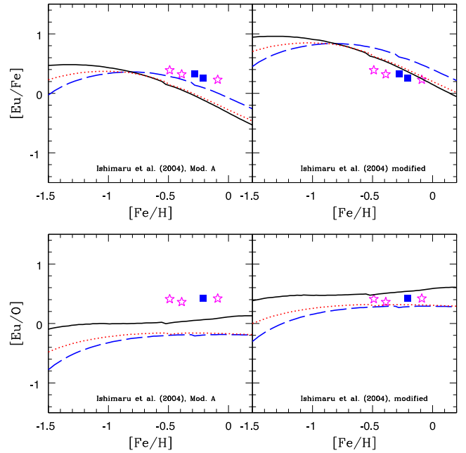
Figure 12. In the top- and bottom-left figures, we compare the predictions of our models with different IMFs for the [Eu/Fe] and [Eu/O] versus [Fe/H] abundance patterns, when the yield of Ishimaru et al. (2004) are included. The latter assume the Eu to be produced by stars with mass in the range M = 8\text{--}10 M_{\odot} , which explode as core-collapse SNe. None of the models with these yields is able to reproduce both the [Eu/Fe] and [Eu/O] abundance ratio patterns at the same time. In the top- and bottom-right figures, we show the predictions of our models when the Eu yields of Ishimaru et al. (2004) are multiplied by a factor of 3; in this case, we can obtain a better results both for the [Eu/Fe] and the [Eu/O] abundance ratios, which can be reproduced by the model the IGIMF. The various lines correspond to the same IMFs as in Fig. 3.
