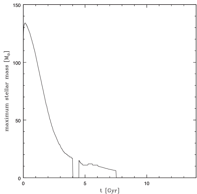
Figure 4. Given the temporal evolution of the SFR and of the [Fe/H] abundance predicted by our chemical evolution model, this figure reports how the maximum stellar mass that can be formed at every time t evolves as a function of the time itself, when assuming the metallicity-dependent IGIMF of R14. It is clear how much the truncation becomes important when the IGIMF is adopted in a detailed chemical evolution model of a galaxy with very low SFRs.
