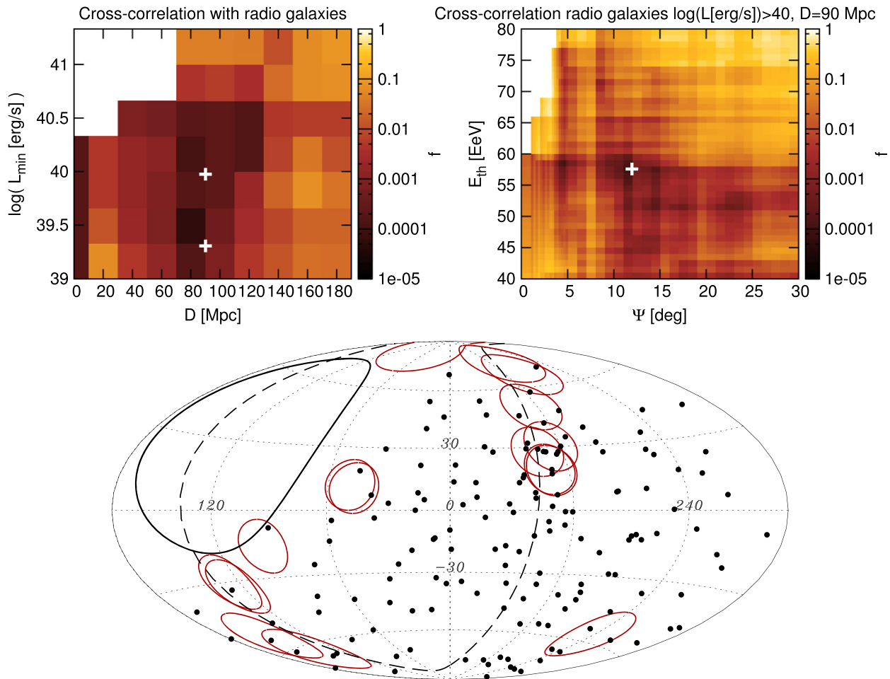
Figure 9. Cross-correlation of events with the radio galaxies as a function of D and L_{\min} (top-left panel) and detail of the scan in \Psi and E_{\text{th}} for the second minimum found (top-right panel). The bottom map (in Galactic coordinates) shows the events with E \geq 58 EeV together with the radio galaxies brighter than 10^{40} erg s ^{-1} and closer than 90 Mpc, indicated with red circles of 12^\circ radius (i.e., the parameters of the second minimum).
