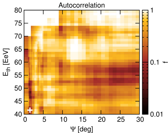
Figure 2. Fraction f obtained in the autocorrelation of events vs. \psi and E_{th} .
