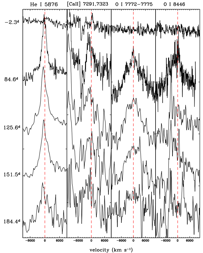
Figure 6. From the left to the right: evolution of the profiles of He I \lambda 5876 , [Ca II] \lambda\lambda 7291,7323 , the O I \lambda\lambda 7772\text{--}7775 and O I \lambda 8446 . The numbers on the left indicate the phases of the spectra from the maximum light.
