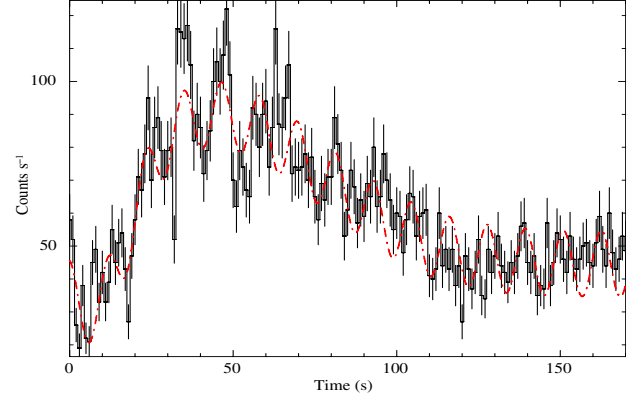
Fig. 5. Swift /XRT WT (0.3–10 keV) light curve (black) fitted with a model consisting of a constant plus two Gaussian for the continuum, and an additional sinusoidal component to account for the modulation.
