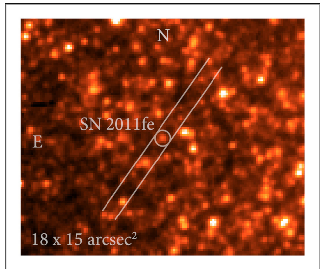
Figure 1. 18 \times 15 arcsec 2 section of an i' -band image, taken with the Gemini-N Telescope + GMOS-N four days after our LBT spectrum. North is up, east to the left. The width and orientation of the 1 arcsec slit used for the LBT observations are indicated.
