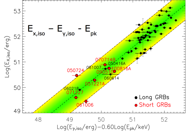
Fig. 1. The E_{X,iso} - E_{\gamma,iso} - E_{p,i} correlation proposed by Bernardini et al. (2012) and Margutti et al. (2013) (courtesy R. Margutti).
