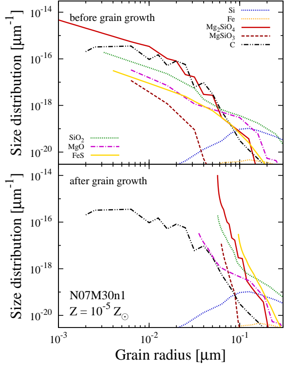
Figure 7. Size distribution function n_i \varphi_i / n_{\text{H}} of dust species i before ( n_{\text{H}} = 0.1 \text{ cm}^{-3} ) and after ( n_{\text{H}} = 10^{16} \text{ cm}^{-3} ) grain growth for our N07M30n1 model with Z = 10^{-5} Z_{\odot} . Size of all species but for C and Si grains increases by accretion of heavy elements. C and Si grains do not grow because the key species, C and Si atoms, are depleted onto CO and SiO molecules, respectively.
