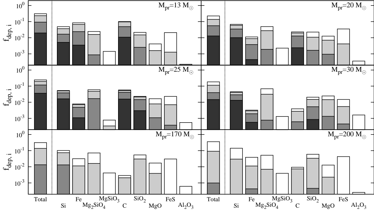
Figure 3. Mass fraction f_{\text{dep},i} of grain species i relative to the total metal mass for supernova model of N07. Each histogram represents the mass fraction for n0, n0.1, n1, and n10 model from top to bottom. The first histogram represents the depletion factor f_{\text{dep}} whereas the other histograms show the contribution of each dust species.
