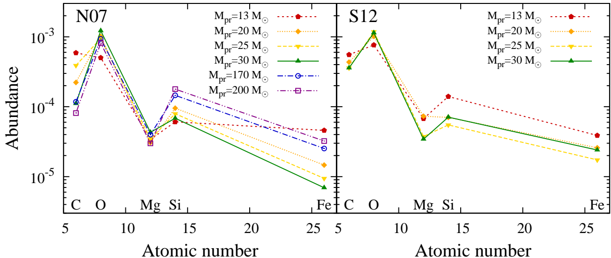
Figure 2. Number abundance A_j of heavy element j for the Pop III supernova models of N07 (left) and S12 (right). We plot the values derived by Equation (1) with Z = Z_{\odot} . For each supernova model, red pentagons, orange diamonds, yellow opposite triangles, green triangles, blue circles, and purple squares show the abundances for supernovae with progenitor masses 13, 20, 25, 30, 170, and 200 M_{\odot} , respectively.
