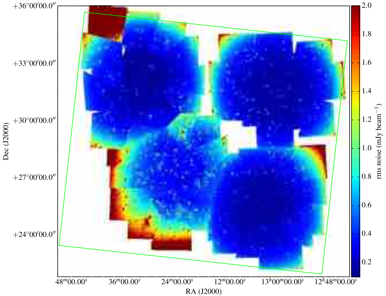
Figure 2. Map showing the sky coverage and rms values of the four fields, constructed as described in the text. Colour levels run from 100 \mu\text{Jy} to 2 mJy \text{beam}^{-1} . The green square shows the approximate boundary of the Herschel survey. The LOFAR survey is deeper (in rms terms) than FIRST, the previous most sensitive radio survey of this area, in the blue regions of the image. The many ‘point sources’ in the image are the result of dynamic range limitations around bright objects, rather than the objects themselves: the pixel size in this image is 20 arcsec, significantly larger than the image resolution.
