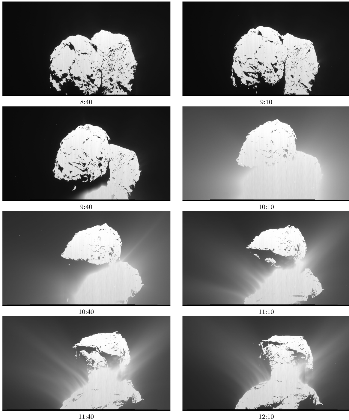
Figure 3. OSIRIS WAC images taken at 08:40, 09:10, 09:40, 10:10, 10:40, 11:10, 11:40, and 12:10, respectively. Each image is about 11.5 \times 6.2 in size, they were obtained in the broad-band green filter with 3 s exposure time. The image brightness is scaled according to the square root of the measured flux, with minimum and maximum values of 1.5 \times 10^{-7} (black) and 1.5 \times 10^{-4} \text{ W m}^{-2} \text{ sr}^{-1} \text{ nm}^{-1} (white). The Sun is at the top.
