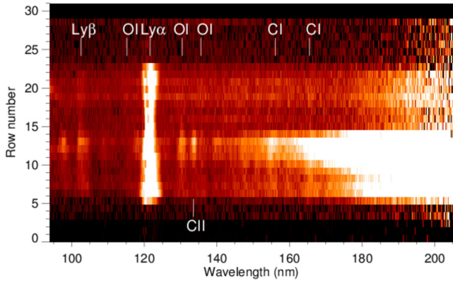
Figure 6. An Alice spectral image beginning at UTC 11:19:44 showing the solar reflected radiation from the nucleus in the lower right. Dust in the coma shows up in the upper right. The orientation of the slit is as shown in Fig. 2. The integration time was 1814 s.
