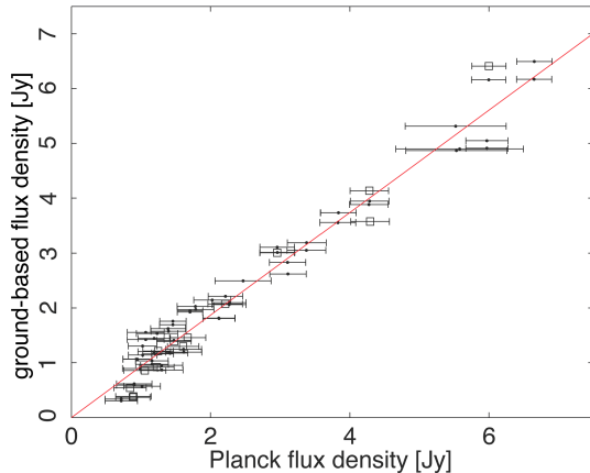
Fig. 4.— Color-corrected (and extrapolated) Planck flux densities compared to VLA measurements ( dots ) and ATCA measurements ( open squares ) of the same sources at 43.34 GHz. The slope and 1\sigma uncertainty of the constrained fit (solid line) are 0.9384 \pm 0.013 .
