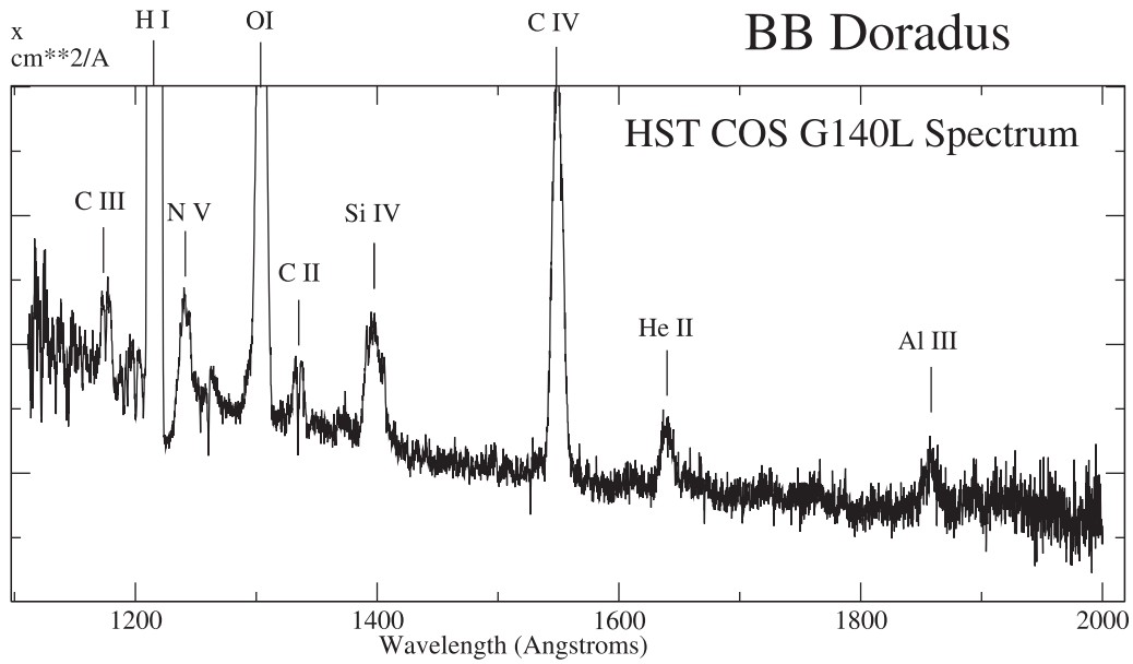
Figure 1. HST/COS spectrum of BB Dor is shown with line identification. The spectrum presents some broad and strong emission lines of high ionization species such as C III (1175 Å), N V (1240 Å), Si IV (1400 Å), and C IV (1550 Å), and also of lower ionization species such as C II (1335 Å) and He II (1640 Å). The hydrogen Ly \alpha (1216 Å) and O I (1302 Å) features are due to geocoronal contamination. Toward the longer wavelengths, after 1700 Å and especially after 1900 Å, there are additional weak but broad emission features that remain unidentified. The region \lambda > 2000 Å is dominated by noise and has been discarded for clarity. For that reason in the modeling we limit the fitting to \lambda < 1850 Å.
