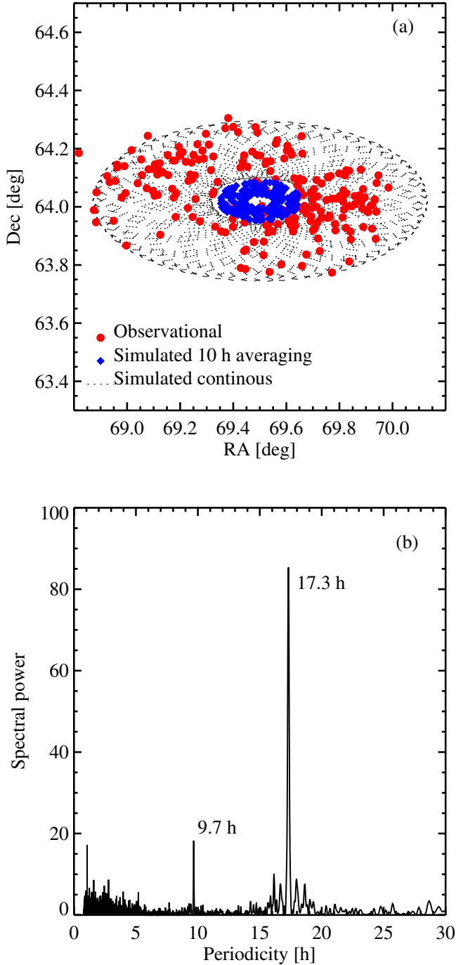
Fig. 6. a) As in Fig. 5, bullets ( \bullet ) show the spin axis orientation as determined with the SPC method (Fig. 2). Small dots ( \cdot ) are the spin vector orientation for a simulated body with inertia moments equal to those derived from the shape of 67P assuming homogeneity, and an E_l = 1.9 \times 10^{-6} under case 1 assumptions, that is, exactly the same circumstances as those of the simulation shown in Fig. 5a. These data are displayed with a time separation of 1 h. Diamonds ( \blacklozenge ), to be compared with the bullet distribution and also with Fig. 5a, correspond to the simulated spin axis orientation at the moments associated with each determination with the SPC method, but now calculated as the average value of the instantaneous coordinates within intervals of 10 h around these moments. b) Lomb periodogram of the simulated averaged Dec coordinates (diamonds) shown in Fig. 6a.
