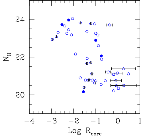
Figure 3. Column density versus the radio core dominance parameter R_{\text{core}} estimated at 5 GHz. Filled points have an R_{\text{core}} estimated at 1.4 GHz.
