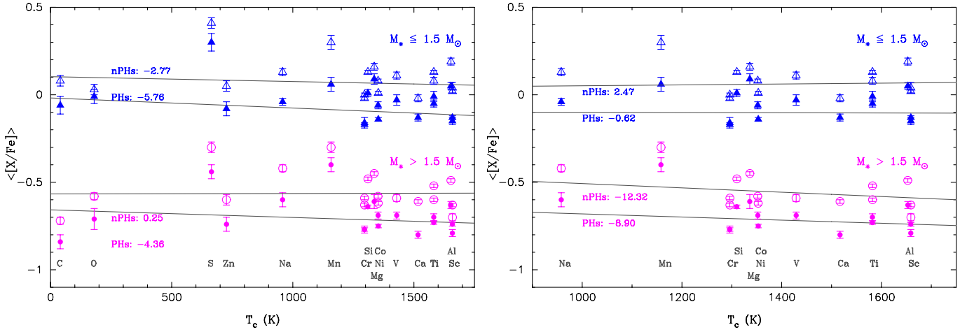
Fig. 7. \langle[X/Fe]\rangle - T_C trends for giant stars. GWPs with M_\star > 1.5 M_\odot are plotted with purple circles, GWPs less massive than 1.5 M_\odot in blue triangles. Filled symbols indicate planet hosts. Each planet host subsample is shown against its corresponding comparison subsample with an offset of -0.15 for the sake of clarity. The offset between the sample of giants with M_\star > 1.5 M_\odot and less massive giants is -0.75 . For guidance, the derived slopes are shown in the plots (units of 10^{-5} dex/K). The left panel shows the \langle[X/Fe]\rangle - T_C trends when all elements (volatiles and refractories) are taken into account, whilst the one on the right shows the \langle[X/Fe]\rangle - T_C trends when only refractories are considered.
