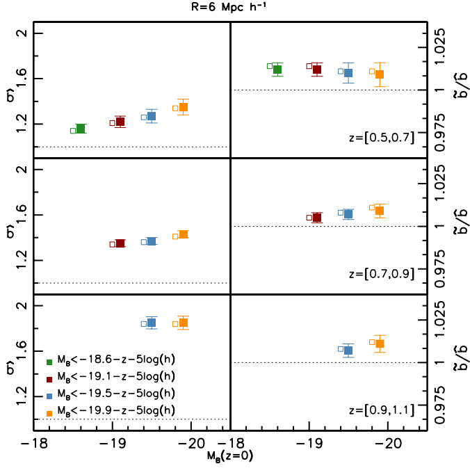
Fig. 9. Second-order moments of the mean biasing functions shown in Fig. 7. Left panels: moment \hat{b} . Right panels: non-linear parameter \hat{b}/\bar{b} . The cell size is R = 6 h^{-1} Mpc. Error bars indicate 1\sigma scatter from the mocks. The redshift ranges and colour code are the same as in Fig. 7. Magnitude cuts are indicated in the plots. All values were computed assuming \sigma_8 = 0.9 . The horizontal dashed line is plotted for reference and represents the case of no bias ( left plot ) and linear bias ( right panels ). Large filled symbols refer to measurements performed at \delta_{\text{MAX}} , and small, open symbols refer to estimates at \bar{\delta}_{\text{MAX}} .
