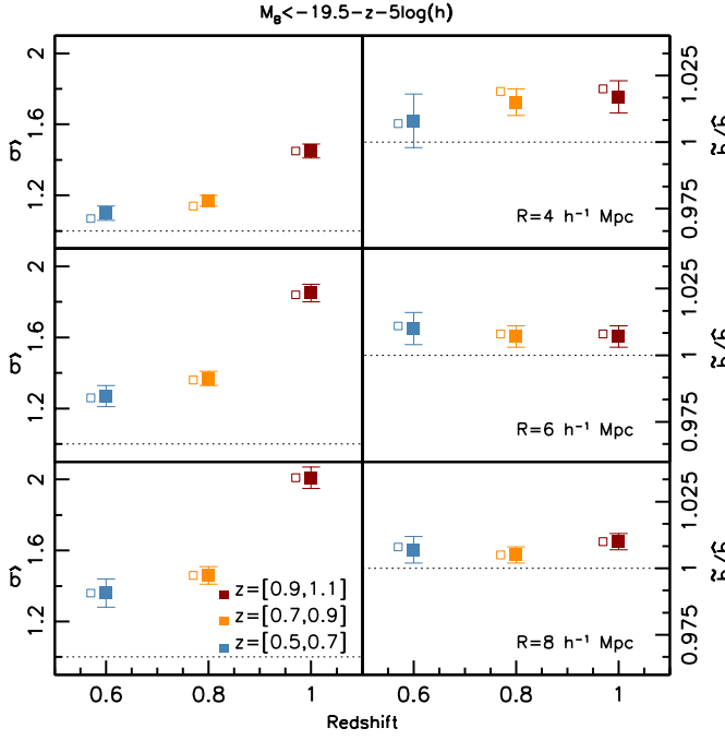
Fig. 12. Moments of the mean biasing functions shown in Fig. 11. Panels from top to bottom indicate cells of increasing size. Left panels: \hat{b} . Right panels: \hat{b}/\bar{b} . Error bars indicate the 1\sigma scatter from the mocks. All values were computed assuming \sigma_8 = 0.9 . Large filled symbols refer to measurements performed at \delta_{\text{MAX}} , small open symbols refer to estimates at \delta_{\text{MAX}} .
