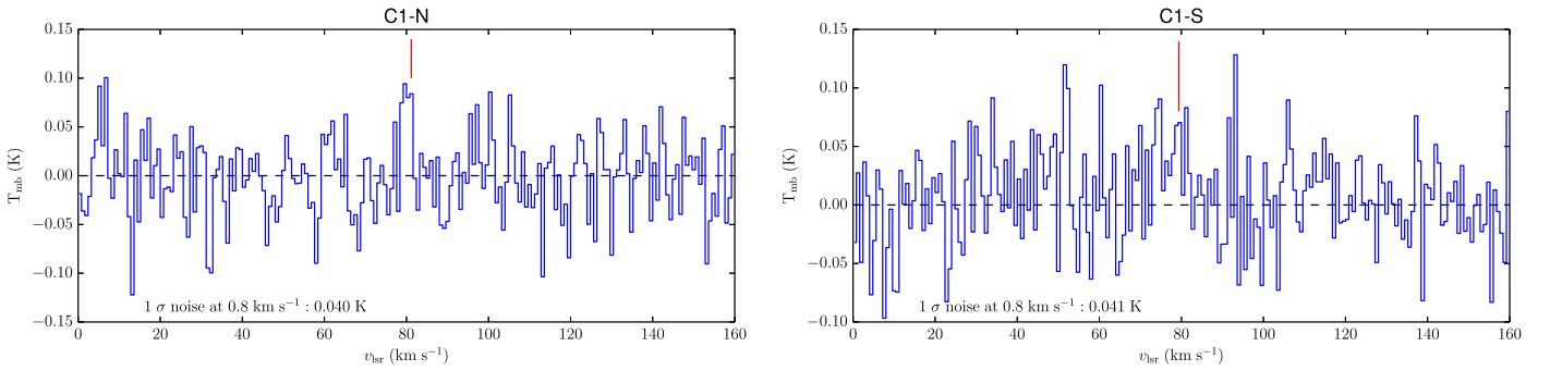
Figure 5. o-H 2 D + spectra for C1-N and C1-S. The binned velocity resolution is 0.8 km s -1 to potentially maximize S/N, considering the total width of N 2 D + spectra from ALMA are ~0.9 km s -1 . The red vertical lines mark the v_{\text{LSR}} of the cores. rms noise levels are labeled in the figure panels.
