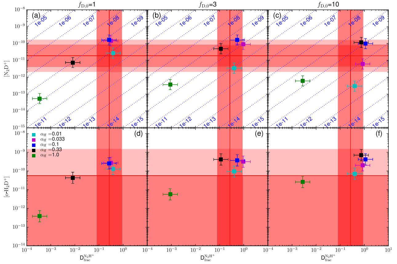
Figure 8. C1-N fiducial models and observational constraints in the [\text{N}_2\text{D}^+]-D_{\text{frac}}^{\text{N}_2\text{H}^+} (top row) and [\text{o-H}_2\text{D}^+]-D_{\text{frac}}^{\text{N}_2\text{H}^+} (bottom row) parameter space. The blue dotted lines in the top row show constant [\text{N}_2\text{H}^+] values. The three columns show different initial depletion factors, f_{D,0} = 1, 3, 10 , for the fiducial astrochemical models, the results of which are indicated by the squares, with different colors representing different collapse rate parameter values ( \alpha_{\text{ff}} = 0.01-1 ; see the legend). Factor of two systematic theoretical errors are indicated by the error bars around each point. All models are evolved to the final, observed density starting from a 10 times lower density, and the initial ortho-to-para ratio of \text{H}_2 is set to one in all of these cases. The red shaded areas show the same observational constraints as described in Figure 6. Fast collapsing \alpha_{\text{ff}} = 1 models are not able to reach the large observed values of D_{\text{frac}}^{\text{N}_2\text{H}^+} (see the text).
