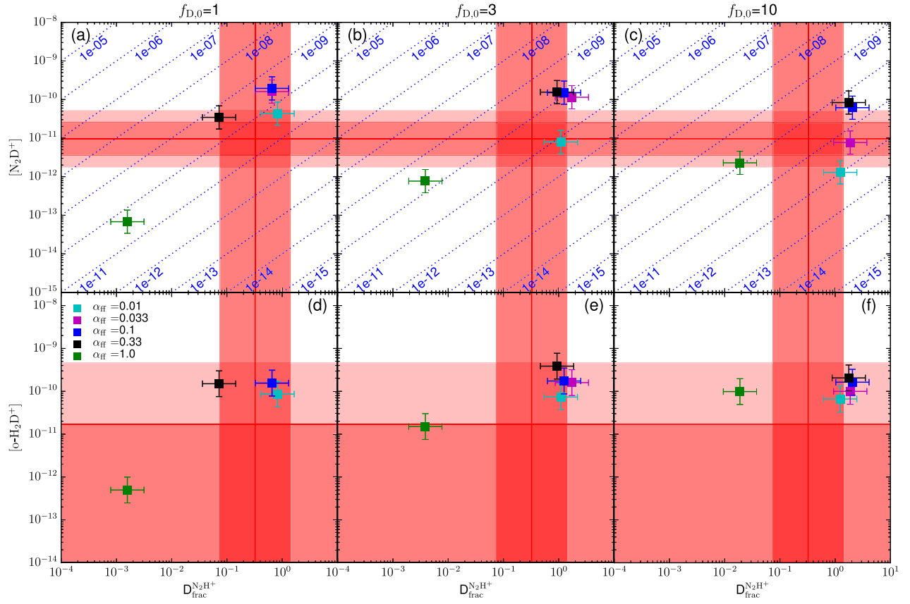
Figure 15. C1-S with low initial ortho-to-para ratio of H 2 , i.e., the same as Figure 14, but for C1-S.
