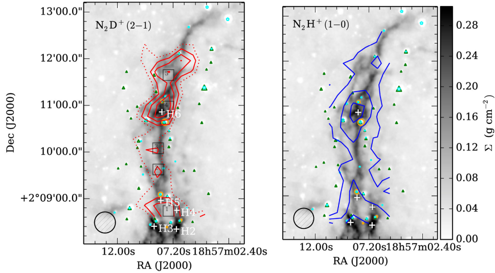
Figure 2. The left-hand panel shows the integrated intensity map of \text{N}_2\text{D}^+ (2–1) emission seen in contours of 2\sigma (dotted panel), 3\sigma , 4\sigma , and 5\sigma ; where \sigma = 0.07 \text{ K km s}^{-1} . Overlaid are boxes which represent the positions of the spectra shown in Fig. 1. The right-hand panel shows the integrated intensity contours of the \text{N}_2\text{H}^+ (1–0) emission, data taken from Paper IV; contours are 5\sigma , 10\sigma , and 15\sigma , where \sigma \sim 0.11 \text{ K km s}^{-1} . Each contour map is overlaid on the mass surface density map (Kainulainen & Tan 2013). White crosses indicate the positions of the massive cores (Butler & Tan 2012), and the symbols indicate the positions of the 8 \mu\text{m} and 24 \mu\text{m} sources (green triangles and cyan pentagons, respectively; Carey et al. 2009), and the 4.5 \mu\text{m} extended emission sources or ‘green fuzzies’ (orange circles; Chambers et al. 2009). The size of each source represents the strength of the emission (Paper I). The hatched circle represents the effective spatial resolution of the observations (after smoothing).
