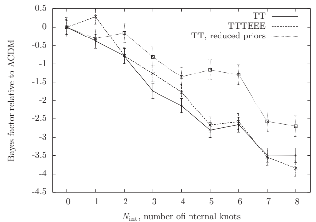
Fig. 25. Bayes factor (relative to the base \Lambda CDM model) as a function of the number of knots for three separate runs. Solid line: Planck TT. Dashed line: Planck TT, TE, EE. Dotted line: Planck TT, with priors on the \mathcal{P}_i parameters reduced in width by a factor of 2 ( 2.5 < \ln(10^{10}\mathcal{P}_i) < 3.5 ).
