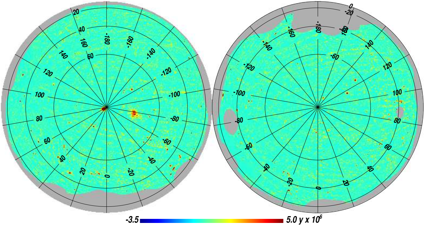
Fig. 19. Orthographic projection of the reconstructed Planck all-sky y-map in Compton parameter units (Planck Collaboration XXII 2015). For illustration purposes and to enhance the tSZ signal-to-noise ratio, the y-map has been Wiener filtered. Positive sources in the map correspond to clusters and super-clusters of galaxies with strong tSZ emission. In particular, the Coma and Virgo clusters are clearly visible near the north Galactic pole. The region of strongest contamination from Galactic foreground emission in the Galactic plane has been partially masked.
