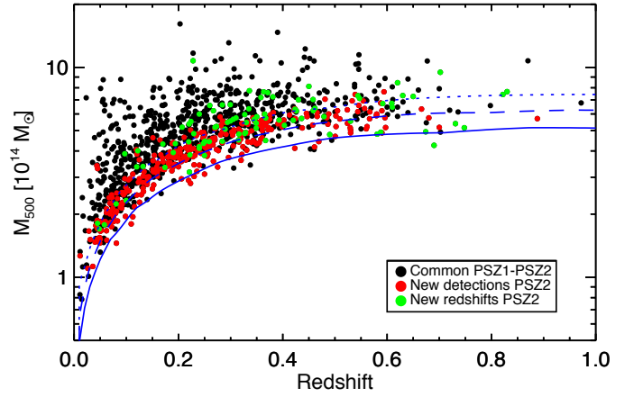
Fig. 14. Distribution of the 1093 PSZ2 clusters with counterparts with known redshift in the M_{500} - z plane. New PSZ2-detected clusters are indicated with red dots, while common PSZ1 and PSZ2 clusters are indicated by black dots. Green dots mark the common PSZ2-PSZ1 detections where we have updated the redshift value for the PSZ2. The solid, dashed, and dotted lines indicate the limiting mass at 20 %, 50 %, and 80 % survey completeness, respectively.
