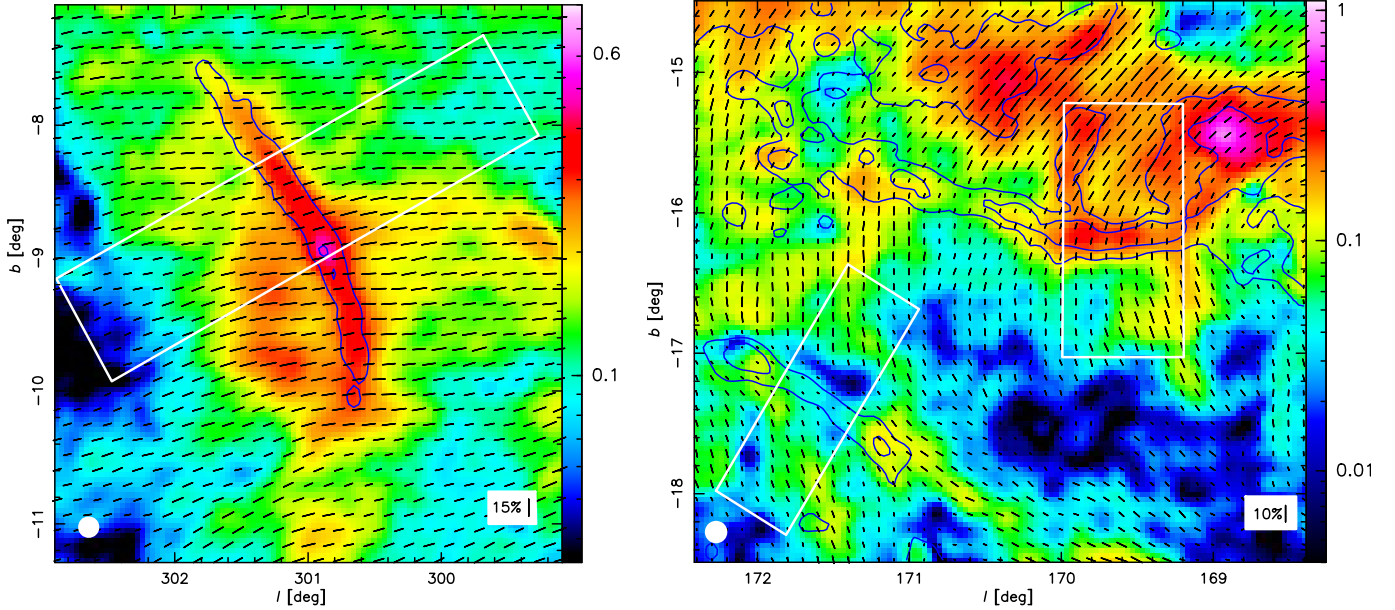
Fig. 7. Observed polarized emission at 353 GHz (in \text{MJy sr}^{-1} ) of the Musca ( left ) and Taurus ( right ) clouds. The maps are at the resolution of 9.6'' (indicated by the white filled circles) for increased S/N. The black segments show the \mathbf{B}_{\text{POS}} -field orientation ( \psi+90^\circ ). The length of the pseudo-vectors is proportional to the polarization fraction. The blue contours show the total dust intensity at levels of 3 and 6 \text{MJy sr}^{-1} , at the resolution of 4.8'' . The white boxes correspond to the area of the filaments and their backgrounds that is analysed in the rest of the paper.
