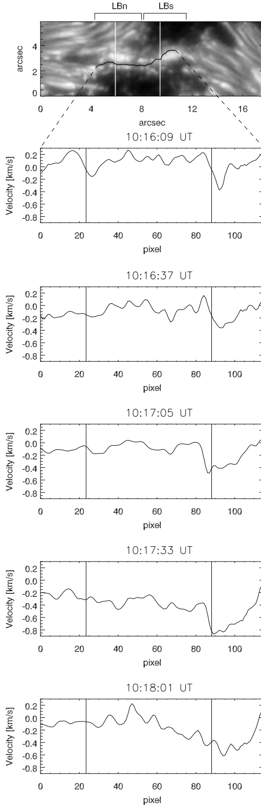
Figure 5. Continuum intensity map from CRISP observations of the LB with an overplotted black line indicating the position of the dark lane studied in the text (top panel) and the LOS plasma velocity values (bottom panels) estimated along the dark lane highlighted on the intensity map. North is on the left of the top image. The two white lines in the top panel and the two black lines in the bottom panel correspond to the lines 1 and 2 reported in Figure 6. Positive (negative) values in velocity indicate motions away from (toward) the observer.
