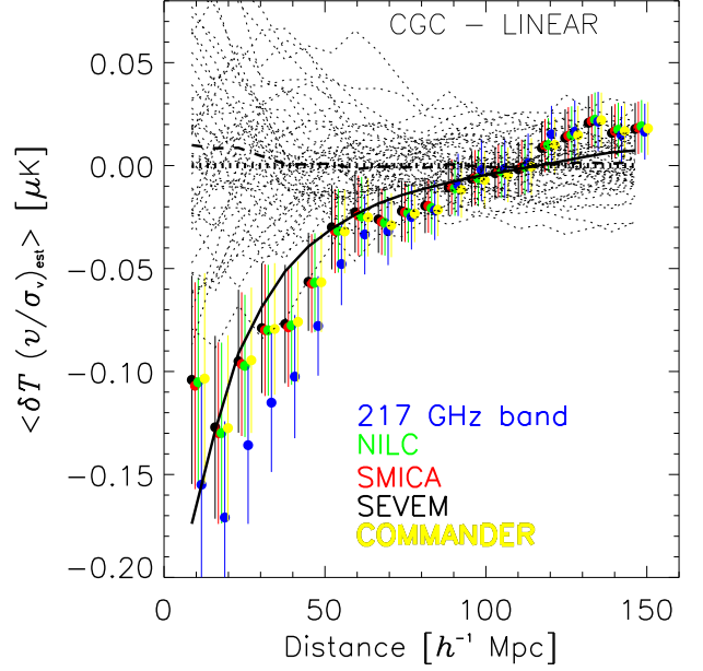
Fig. 6. Measured cross-correlation function between the kSZ temperature estimates and the recovered radial peculiar velocities, w^{T, \nu_{\text{los}}^{\text{rec}}}(r) , according to the LINEAR approach. The recovered velocities are divided with their rms dispersion \sigma_{\nu} = 310 \text{ km s}^{-1} , so kSZ temperature estimates are correlated to a quantity of variance unity. This plot corresponds to an aperture of 8 arcmin. Filled coloured circles correspond to w^{T, \nu_{\text{los}}^{\text{rec}}}(r) estimates from different CMB maps (SEVEM, SMICA, NILC, COMMANDER, and the HFI 217 GHz map). The dotted lines display the null estimates obtained after computing kSZ temperature estimates for rotated positions on the SEVEM map, and the thick dashed line displays the average of the dotted lines. Error bars are computed from these null estimates of the correlation function. The solid line provides the best fit of the SEVEM data to the theoretical prediction for w^{T, \nu_{\text{los}}^{\text{rec}}}(r) obtained from the GALAXY mock catalogue. These predictions are obtained using only a relatively small number of mock halos, and hence their uncertainty must be considered when comparing to the data.
