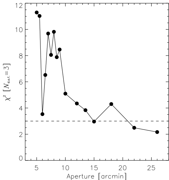
Fig. 9. Evaluations of the \chi^2 statistic of the w^{\text{T},\text{v}_{\text{los}}^{\text{rec}}}(r) correlation function (with respect to the null hypothesis) for different angular apertures. Only results for the foreground-cleaned SEVEM map are shown. There is evidence for kSZ signal in a wide range of apertures above the FWHM, with a local maximum close to 8 arcmin. This roughly corresponds to a radius of 0.8 h^{-1} Mpc from the CG positions at the median redshift of the sample.
