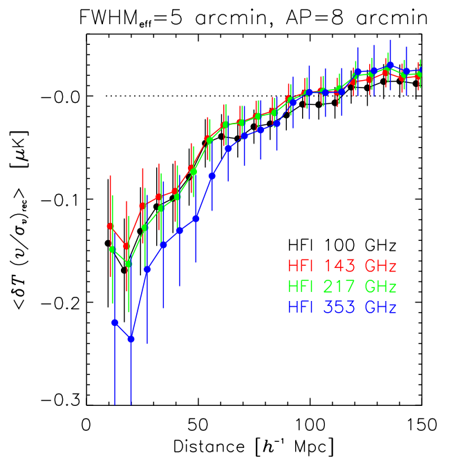
Fig. 10. Variation of the recovered raw HFI maps after an effective convolution by a Gaussian beam of FWHM = 5 arcmin. Error bars here are computed in the same way as in Figs. 6 and 8.
