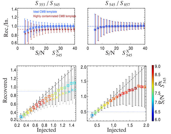
Fig. 10. Colour-colour ratio recovery. Left : S_{353}/S_{545} . Right : S_{545}/S_{857} . Top : ratio of recovered over injected colour-colour ratio (Rec./In.) as a function of the 545 GHz excess S/N. This is shown for two choices of the CMB template, i.e., ideal (blue squares) or highly contaminated by extragalactic foregrounds (red crosses). Bottom : recovered versus injected colour-colour ratio per bin of input colour-colour ratio. Again, two cases are shown depending on the quality of the CMB template, ideal (squares) or highly contaminated (crosses). The colour scale provides the average S/N of the 545 GHz excess inside each bin of input colour-colour ratio. The blue dotted lines show S_{353}/S_{545} < 0.9 and S_{545}/S_{857} > 0.5 , which are the colour criteria adopted for source selection.
