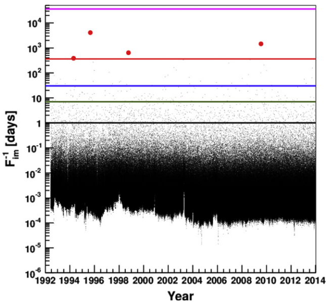
Figure 6. Distribution of detected clusters versus time between 1992 June and December 2013. Red dots represent clusters with imitation frequency less than F_{\text{im}} = 1/\text{year} . Black, green, blue, red, and purple lines correspond to F_{\text{im}}^{\text{th}} = 1/\text{day} , F_{\text{im}}^{\text{th}} = 1/\text{week} , F_{\text{im}}^{\text{th}} = 1/\text{month} , F_{\text{im}}^{\text{th}} = 1/\text{y} , and F_{\text{im}}^{\text{th}} = 1/100 \text{ y} , respectively.
