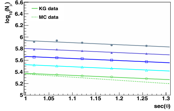
Figure 5. Muon attenuation curves extracted with the CIC method from the experimental KASCADE-Grande data. The result of the global fit with equation (1) is shown with solid lines. The highest curve correspond to the lowest CIC cut. The segmented line is an example of the result from the global fit applied to the EPOS-LHC data (mixed composition scenario with \gamma = -3 ).
