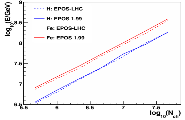
Figure 2. Predictions of EPOS-LHC and EPOS 1.99 for the dependence of the primary energy on N_{ch} for two different primary compositions at the site of the KASCADE-Grande observatory for the respective experimental threshold for secondary particles. No experimental effects on the EAS observables were taken into account. Only showers with \theta \leq 18^\circ were considered.
