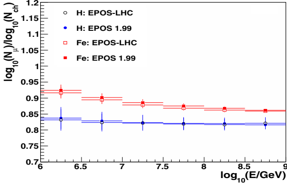
Figure 3. Predictions of EPOS-LHC and EPOS 1.99 for the energy dependence of the ratio \log_{10}(N_{\mu})/\log_{10}(N_{ch}) for EAS generated for different primary compositions. No experimental effects on the EAS observables were taken into account. Only EAS with \theta \leq 18^{\circ} were considered.
