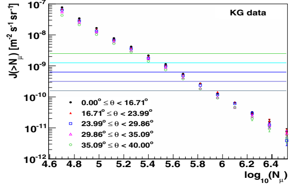
Figure 4. Integral muon fluxes for five zenith angle intervals derived from the measurements with the KASCADE-Grande observatory. The muon correction function was already applied to the data. The CIC cuts employed in this work are shown as horizontal lines. From below to above, the CIC cuts are: \log_{10}[J_{\mu}/m^2 \cdot s \cdot sr] = -9.80, -9.50, -9.20, -8.90, -8.60 .
