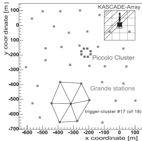
Figure 1. The KASCADE-Grande layout. Different detection systems are shown: the Grande and the KASCADE arrays, the central detector (CD), the Piccolo cluster and the Muon Tracking Detector (MTD).
