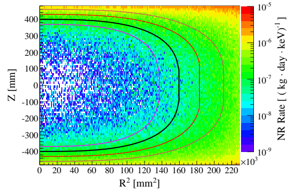
Figure 8. Spatial distribution of the NR background events from radiogenic neutrons inside the active LXe volume, in the (4, 50) keV energy range. The thick black line indicates the reference 1 t super-ellipsoid fiducial volume. In purple, red and brown, we indicate the FV corresponding to 800 kg, 1250 kg and 1530 kg, respectively. The white regions present a background rate smaller than 1 \cdot 10^{-9} \text{ (kg} \cdot \text{day} \cdot \text{keV)}^{-1} .
