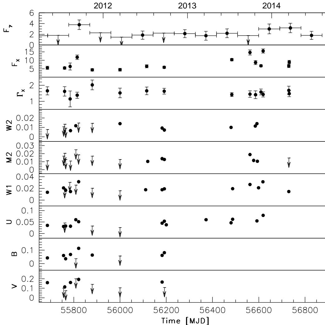
Figure 7. Multifrequency light curve of PKS 2004–447 for the period between 2011 May and 2014 August. The LAT \gamma -ray light curve (in units of 10^{-8} ph \text{cm}^{-2} \text{s}^{-1} for 0.1 < E < 100 GeV; upper panel ), the Swift X-ray light curve (in units of 10^{-13} erg \text{cm}^{-2} \text{s}^{-1} for 0.3 < E < 10 keV; second panel from top ), the X-ray photon index trend ( third panel ), the Swift -UVOT light curve in the optical and UV filters ( v , b , u , w1 , m2 , w2 , in units of mJy; fourth to ninth panel ). Arrows refer to 2\sigma and 3\sigma upper limits on the source flux for LAT and Swift -UVOT measurements, respectively.
