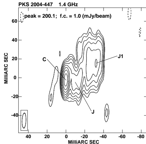
Figure 3. VLBA image at 1.4 GHz of PKS 2004–447. On the image we provide the peak flux density in \text{mJy beam}^{-1} and the first contour intensity (f.c.) in \text{mJy beam}^{-1} , which corresponds to three times the off-source noise level measured on the image plane. Contours increase by a factor of 2. The restoring beam is plotted in the bottom left corner.
