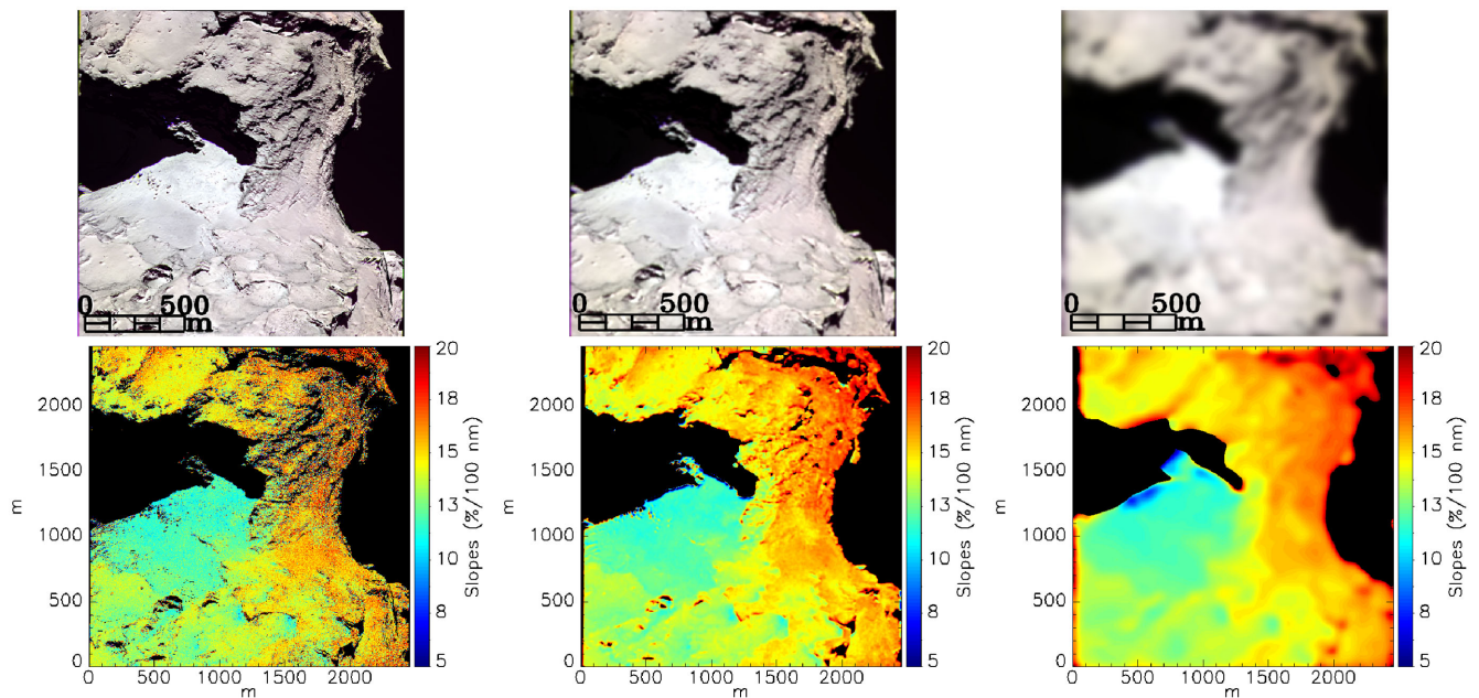
Figure 6. Colour composites (top panels) and corresponding spectral slopes (bottom panel) of Hapi region at original NAC resolution in left-hand panels, DI -HRI resolution in middle panels and DI -MRI resolution in right-hand panels. Images taken in 989.3, 649.2 and 360.0 nm are assigned to the RGB channels of the top panel images, respectively.
