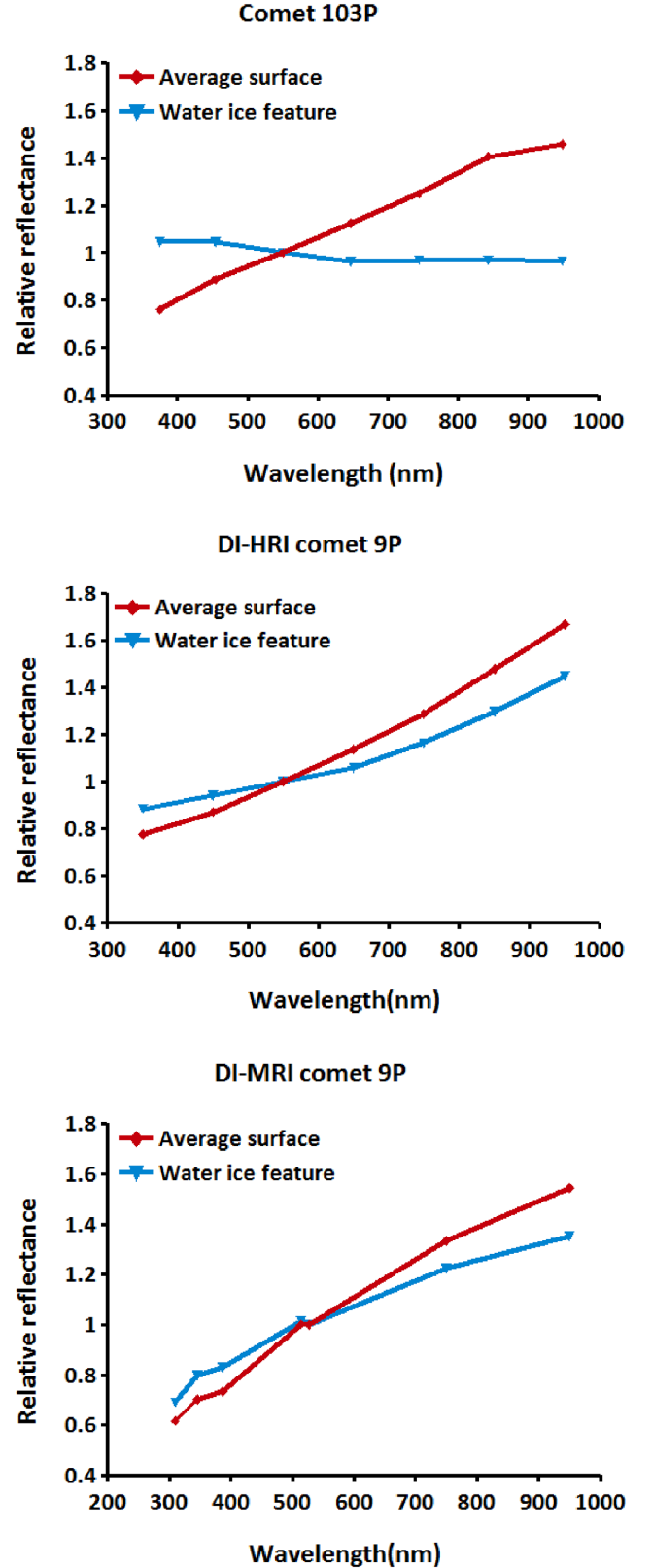
Figure B4. Mean spectra of the water ice deposits (blue patches) seen in Fig. B2 together with the selected mean surface (red rectangles in Fig. B2). Top panel is the relative reflectance of the water ice deposit observed on comet 103P, while middle and bottom panels show the relative reflectance of the water ice deposits observed on comet 9P in DI-HRI and DI-MRI resolutions with the average surface spectra, respectively.
