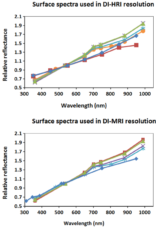
Figure B3. Mean surface spectra considered in this study. Top panel shows the mean surface spectra used in the right-hand column of Fig. 4 and in the top panel of Fig. 7, while the bottom panel shows the mean surface spectra used in the right-hand column of Fig. 5 and in the bottom panel of Fig. 4.
