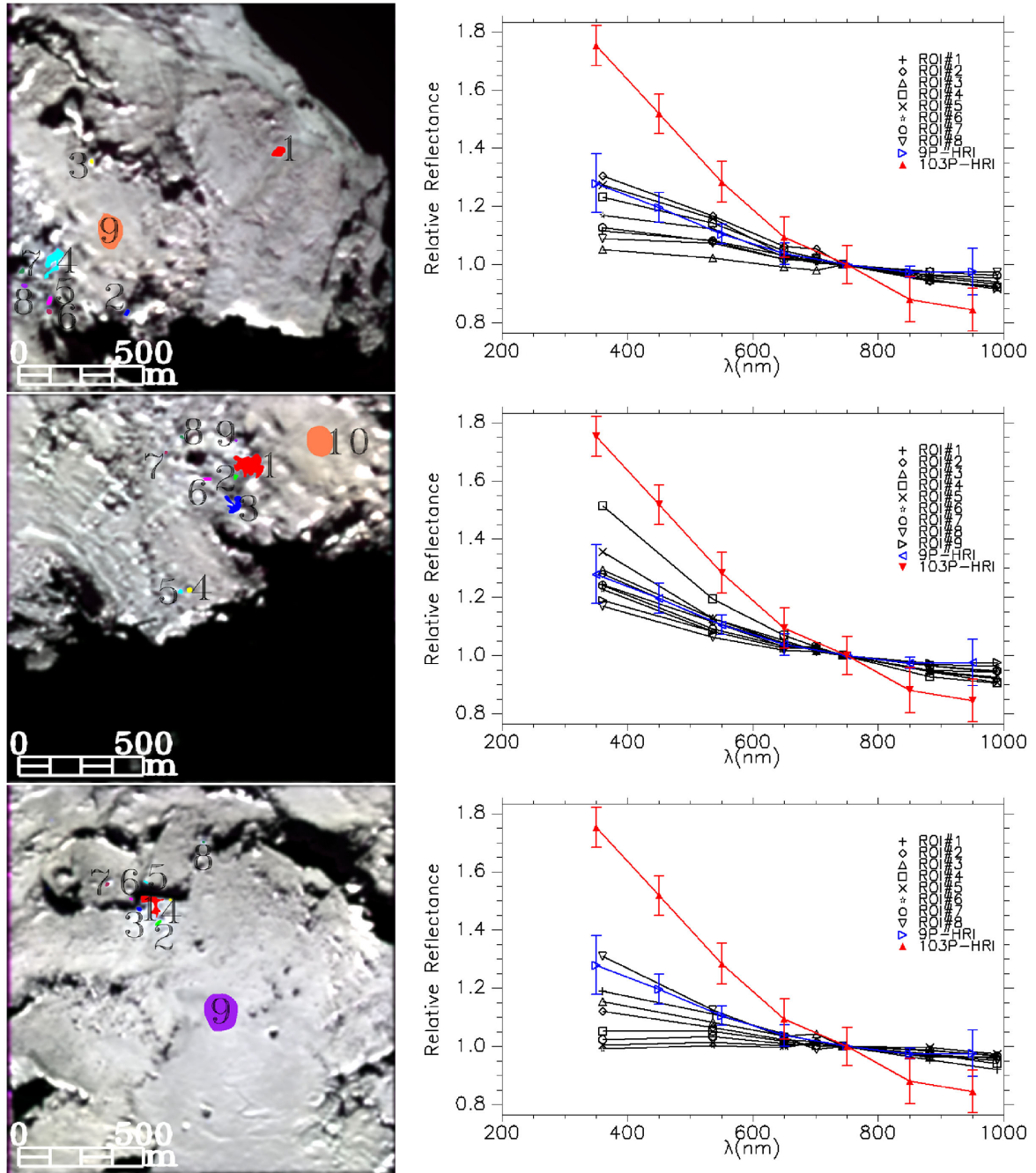
Figure 4. Selected ROIs on the NAC image sets (from top to bottom) in DI -HRI spatial resolution (left-hand panel) with relative reflectance calculated in each ROI (right-hand panel) together with the spectra of water ice deposits observed on comets 9P and 103P. Typical standard deviations of the data points from the resistant mean are 8.93 \times 10^{-5} , 9.64 \times 10^{-5} , 1.44 \times 10^{-4} from top to bottom. The ROIs with largest # represent the average surface, where the mean spectra of each ROI are normalized (see Fig. B3 for the spectra).
