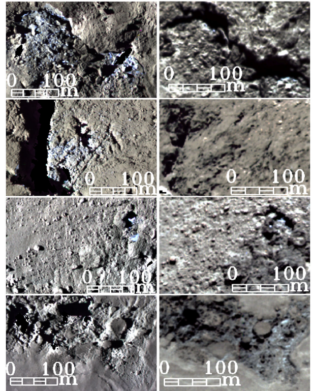
Figure 10. Comparison of the water-ice-rich features observed at two different epochs (Table 2). The images in the left-hand panel are taken on 2014-09-05, while the images in the right-hand panel are taken on 2016-01-24. Images taken in 882.1, 649.2 and 480.7 nm filters are used to generate colour composites. Histogram match stretch is applied to the image pairs. Top two panels are the water-ice-rich clusters BAP2 (top panel) and BAP1 (second panel) of Filacchione et al. (2016c). Third panel from the top shows one potentially water-ice-rich (upper) and one water-ice-rich (lower) feature (Barucci et al. 2016, spot 5). Bottom panels show the roundish features and their surrounding material.
