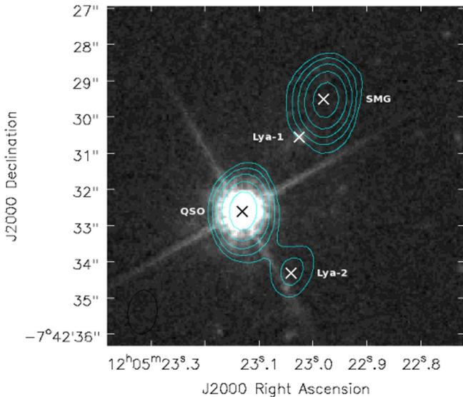
Figure 1. BRI 1202–0725 field. Contours show the 340 GHz continuum from Carilli et al. (2013). Contours are a geometric progression of 2, starting at \pm 4 \times 0.1 \text{ mJy beam}^{-1} , and the beam is 1.2'' \times 0.8'' at PA -7^\circ . The background shows the HST /ACS F775W filter image of Decarli et al. (2014). Positions of each object from 340 GHz are marked, except for Ly \alpha -1, whose optical position is marked.
