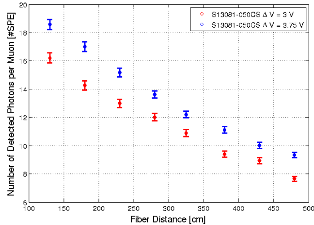
Figure 11. Number of detected photons per muon impinging the detector as a function of the fiber distance for two different overvoltages: \Delta V = 3 V and \Delta V = 3.75 V. The detector light yield is not uniform due to the fiber attenuation. Error bars are only due to statistic errors of the mean. All the measurements were done at 25 °C.
