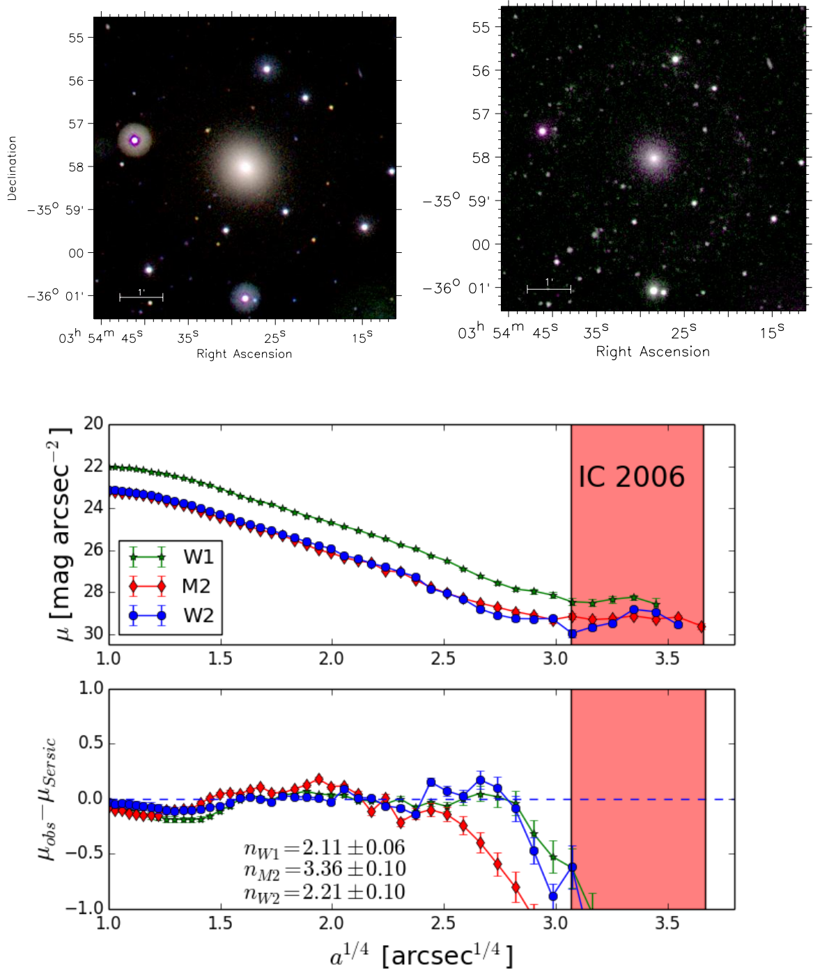
Fig. 14. As in Figure 4 for IC 2006. The field of view is 7'×7'. The shaded area indicates the masked region in the Sérsic law fit (see text).
