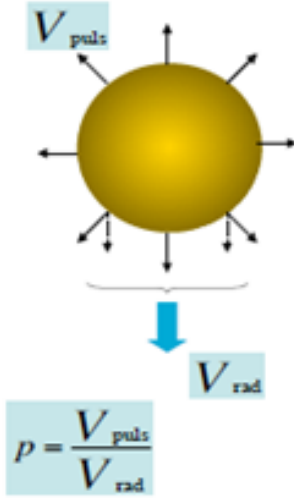
Fig. 1: Graphical representation of the projection factor p between the true pulsational velocity V_{\text{puls}} of the star and the radial velocity V_{\text{rad}} measured by the observer.
