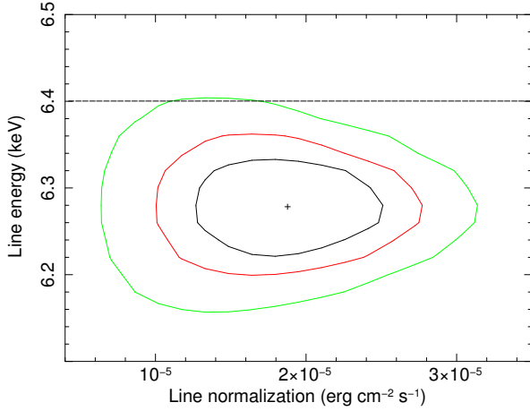
Fig. 5. 68% (black), 90% (red), 99% (green) confidence contours. The two-dimensional confidence contours allow a marginal consistency with the iron K \alpha line at 6.4 keV, indicated by the dashed horizontal line.
