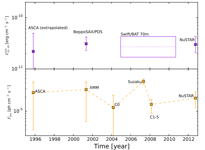
Fig. 9. Observed 10–40 keV flux ( top panel ) and iron line flux ( bottom panel ) of Mrk 1210, as a function of time.
