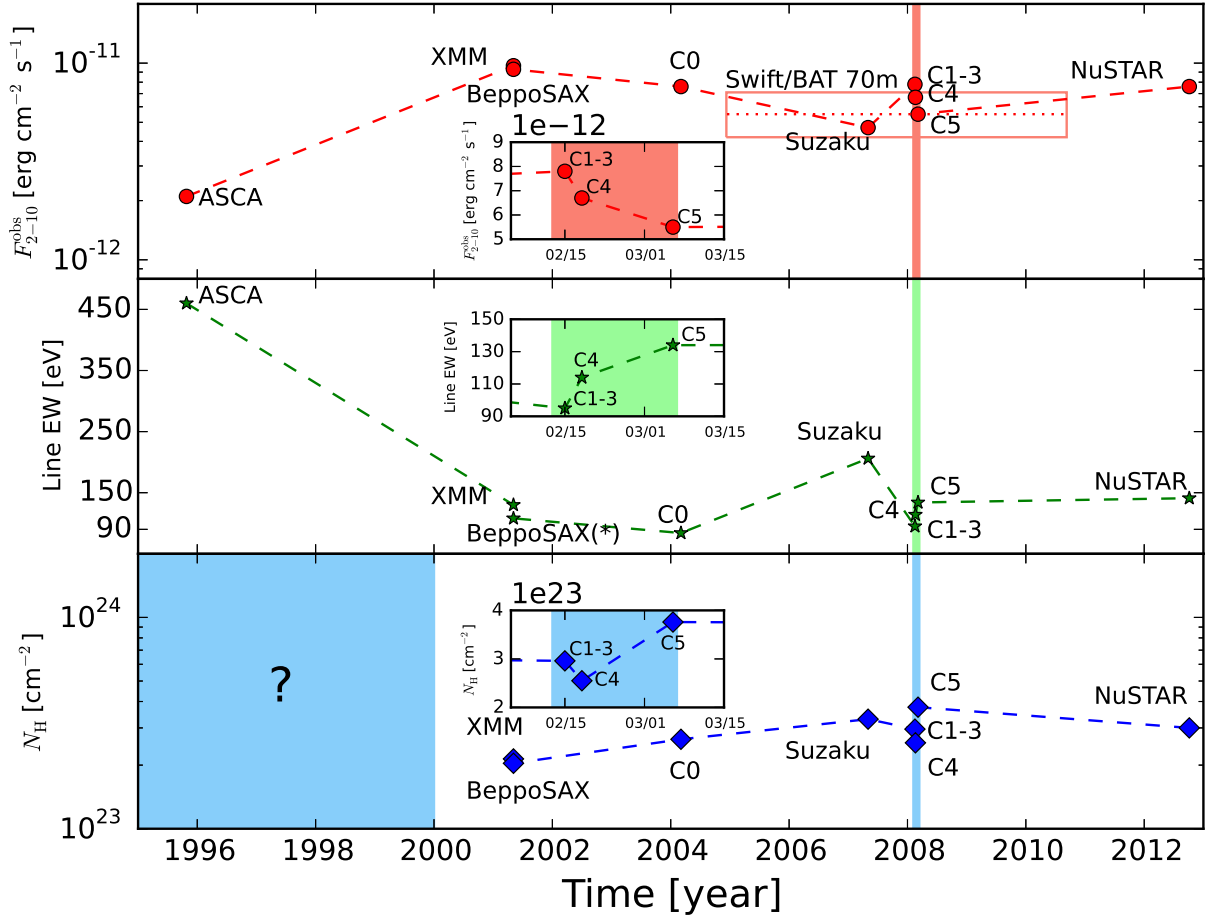
Fig. 8. Observed flux in the 2–10 keV band of Mrk 1210 ( top panel ), Fe K \alpha line equivalent width ( middle panel ) and column density ( bottom panel ) as a function of time. The inset panels show the zoomed-in region of the five Chandra observations during 2008. (*) We report here the equivalent width of model 1 instead of that of model 2 in Ohno et al. (2004). The two values are consistent within the uncertainties, and we adopt the more constrained one for clarity.
