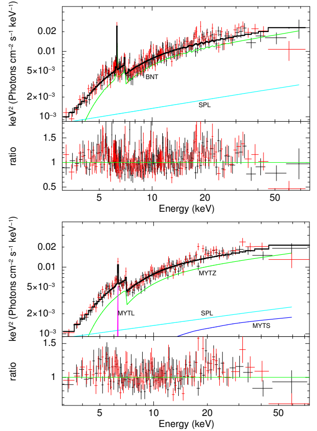
Fig. 6. Fit with the BNTorus model ( top ) and the coupled MYTorus model ( bottom ) to the NuSTAR spectrum of Mrk 1210 (FPMA in black, FPMB in red).
