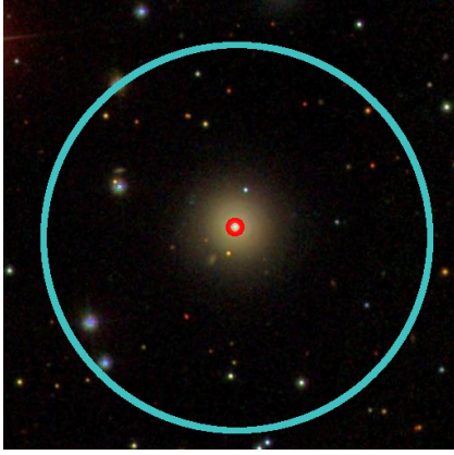
Fig. 1. Sloan Digital Sky Survey (SDSS) optical image of Mrk 1210 (grayscale composite). The cyan and red circles are the source extraction regions for the NuSTAR (see Sect. 2) and Chandra (see Appendix A) spectra, respectively.
