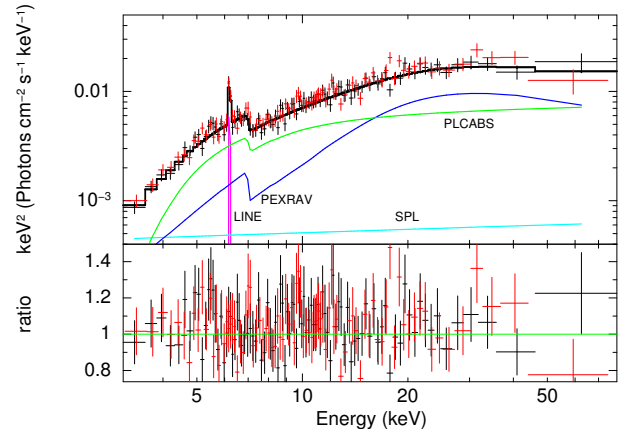
Fig. 4. Fit with the baseline model (1) to the NuSTAR spectrum of Mrk 1210 (FPMA in black, FPMB in red).
