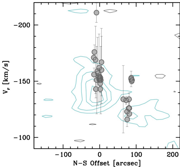
Figure 4. A position–velocity slice along the north–south direction of the H I data by A15 is compared with the velocity of the H II regions identified in this paper (grey filled circles). The H I intensity contours are plotted at -2 (black), 2 , 4 , 6 and 8 (green) \text{mJy bm}^{-1} .
