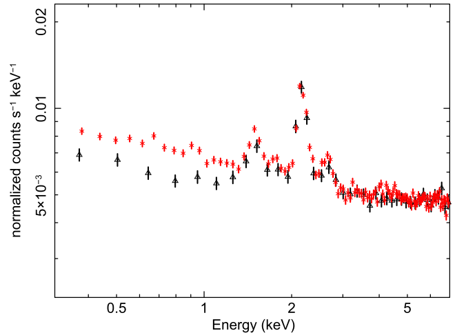
Figure 1. Comparison of the nsCXB (red stars) before background subtraction and the PIB (black triangles). It is worth noting that the error bars of the PIB spectrum are much larger than those of the raw nsCXB spectrum.
