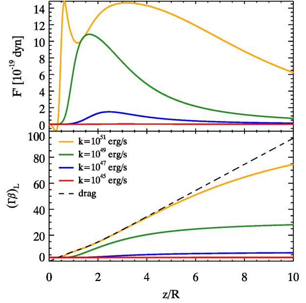
Figure 3. Radiative acceleration of the layer by varying k_L = L_{\text{iso},S} \cdot \langle\gamma_L^2\rangle (values from 10^{45} to 10^{51} erg s ^{-1} ). The spine Lorentz factor is constant \Gamma_S = 15 . The initial Lorentz factor of the layer is \Gamma_{L,0} = 3 . The x-axis is common for the two panels and depicts the position z normalized by the vertical structure dimension R . Top panel: radiative force F' as measured in the frame of the layer as a function of z/R . Bottom panel: layer Lorentz factor (\Gamma\beta)_L (solid lines) and the drag Lorentz factor (\Gamma\beta)_{L,\text{drag}} of the layer (dashed line) as a function of z/R .
