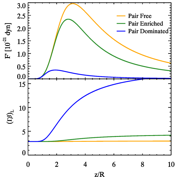
Figure 14. Radiative acceleration of a cold, pair–loaded layer plasma by varying lepton to proton ratio f ; we analyze three cases with \langle \gamma^2 \rangle = 1 : no pairs in layer ( f = 1 ); a plasma with f = 20 and the extreme case of a pair dominated plasma. Parameters used: \Gamma_S = 15 , \Gamma_{L,0} = 3 and L''_S = 10 \cdot L'_L . Top panel: radiative force as measured in the layer frame. Bottom panel: profile of (\Gamma\beta)_L for the layer.
