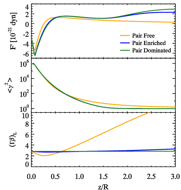
Figure 15. Radiative acceleration plot for a hot layer plasma having different lepton to proton ratios f ; we analyze three distinct cases with an initial \langle \gamma^2 \rangle_{z=0} = 10^6 : no pairs in layer and spine plasma ( f = 1 ); a pair–enriched f = 20 plasma, and the extreme case of a pair dominated plasma. Parameters used: \Gamma_S = 15 , \Gamma_{L,0} = 3 and L''_S = 10 \cdot L'_L . Top panel: radiative force measured in layer frame as a function of z/R . Middle panel: the evolution of internal energy of the sheath denoted by \langle \gamma_L^2 \rangle . Bottom panel: profile of (\Gamma\beta)_L for the layer as a function of z .
