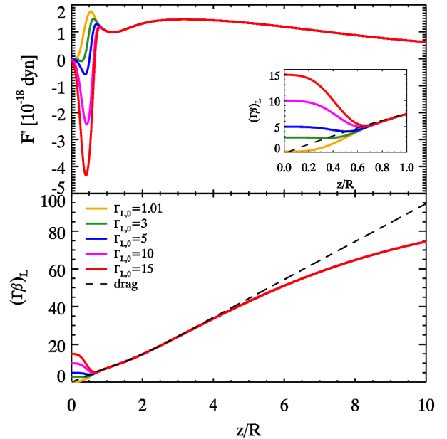
Figure 4. Radiative acceleration of the layer obtained by varying the initial layer Lorentz factor \Gamma_{L,0} = 1.01, 3, 5, 10, 15 . The spine isotropic luminosity is L_{\text{iso},S} = 10^{45} erg/s and the leptons of the layer are hot ( \langle\gamma_L^2\rangle = 10^6 ) implying k_L = 10^{51} erg/s. The spine Lorentz factor is constant \Gamma_S = 15 . Top panel: radiative force F' in layer frame as a function of z/R . Bottom panel: layer Lorentz factor (\Gamma\beta)_L (solid lines) and the drag Lorentz factor (\Gamma\beta)_{L,\text{drag}} of the layer (dashed line) as a function of z/R ; Inset: a zoomed view of the behaviour of the layer Lorentz factor for 0 < z/R < 1 .
