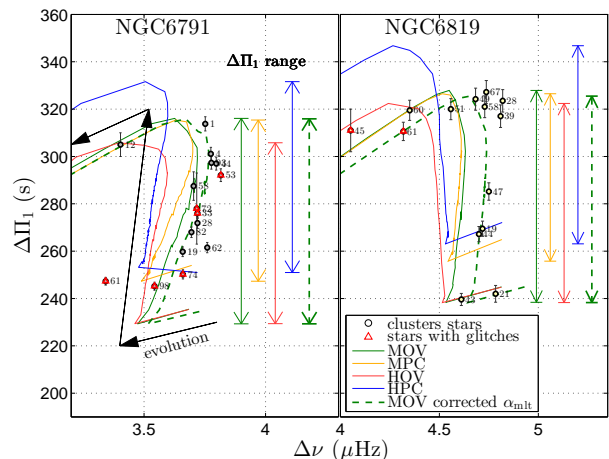
Figure 1. Red-clump stars in NGC6791 and NGC6819 in a \Delta\Pi_1 - \Delta\nu diagram. Model predictions based on different near-core mixing schemes are shown by solid lines. The vertical lines indicate the range of \Delta\Pi_1 covered by each mixing scheme. The dashed line shows MOV models computed with slightly ( \lesssim 3\% ) increased mixing-length parameters (compared to the solar-calibrated value). The red triangles mark the presence of buoyancy glitches which, to the first order, induce a modulation in \Delta\Pi_1 with respect to the asymptotic value (Miglio et al. 2008, Cunha et al. 2015, and Fig. 10 of Mosser et al. 2015), potentially hampering an accurate inference of the asymptotic \Delta\Pi_1 .
