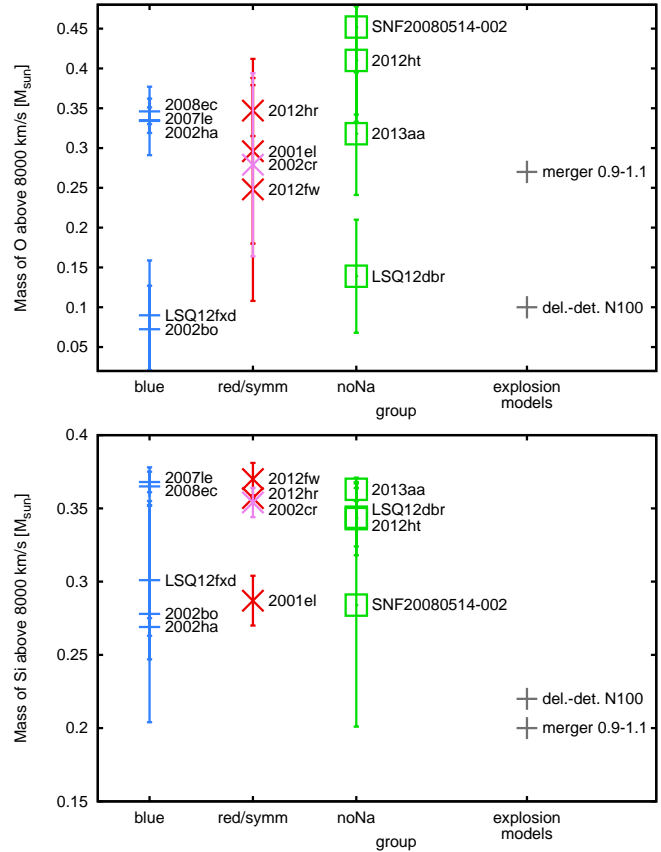
Figure 7. Mass of O ( upper panel ) and Si ( lower panel ) above 8000 \text{ km s}^{-1} in our models, which are grouped according to the narrow Na 1D line behaviour of the corresponding SN (left three columns, respectively). The error bars correspond to the error in v_{\text{ph}} ( \pm 1000 \text{ km s}^{-1} , as in Figure 6). For comparison, we plot the corresponding masses within the hydrodynamical explosion/nucleosynthesis models of Röpke et al. (2012) (right column within each panel). The variations in Si mass are actually relatively small (fine mass scale in lower panel) both among our SNe and the hydro models. The merger model ‘compensates’ for its smaller Fe-group mass in the outer layers (Figure 6) by having a larger O abundance and a significant amount of unburned C ( \sim 0.1 M_{\odot} , not plotted).
