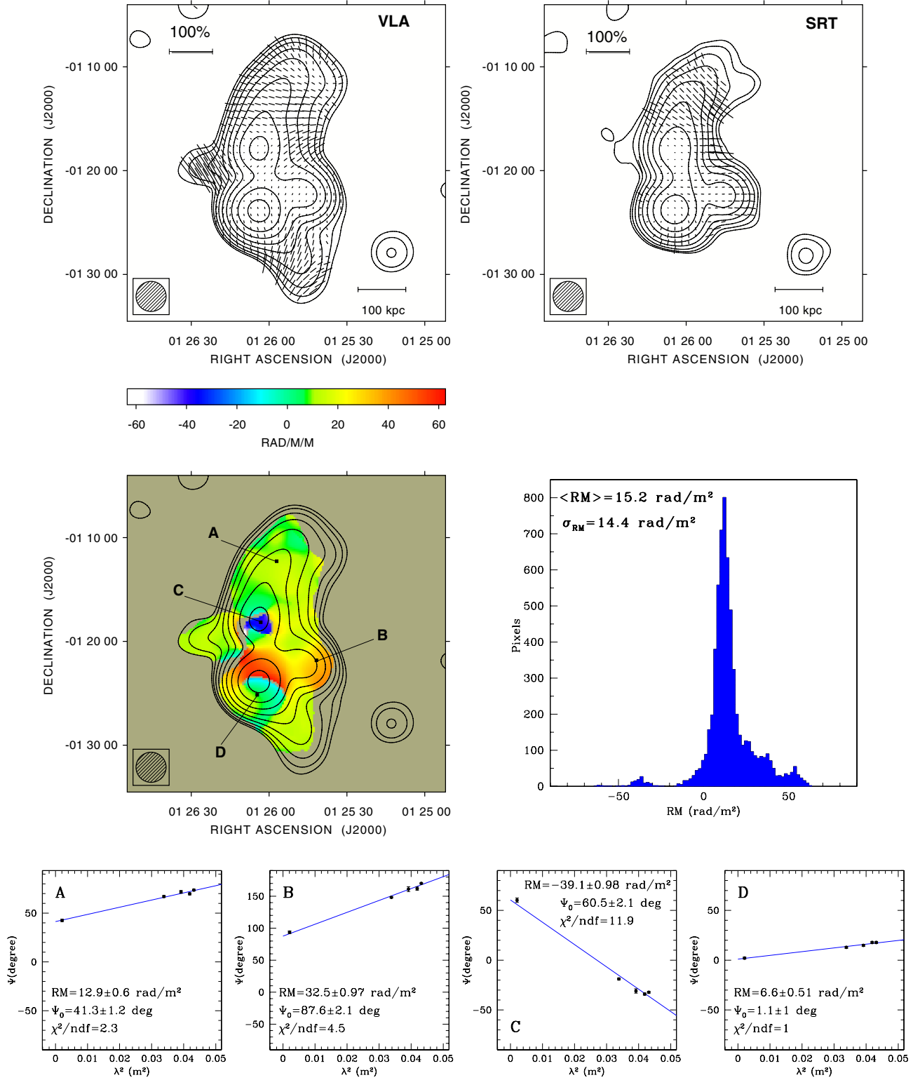
Fig. 8. Top: total intensity contours and polarization vectors of the radio sources in Abell 194. VLA image ( left ) at 1443 MHz ( \sigma_1 = 2 \text{ mJy/beam} ), smoothed with a FWHM Gaussian of 2.9'' . SRT image ( right ) at 6600 MHz ( \sigma_1 = 1 \text{ mJy/beam} ), with a resolution of 2.9'' . The radio contours are drawn at 3\sigma_1 and the rest are spaced by a factor of 2. The lines give the orientation of the electric vector position angle (E-field) and are proportional in length to the fractional polarization. The vectors are only traced for those pixels where the total intensity signal is above 5\sigma_1 , the error on the polarization angle is less than 10^\circ , and the fractional polarization is above 3\sigma_{\text{FPOL}} . Middle left: RM image calculated using the images at 1443, 1465, 1515, 1630, and 6600 MHz, smoothed with a FWHM Gaussian of 2.9'' . The color range is from -60 to 60 \text{ rad/m}^2 . Contours refer to the total intensity image at 1443 MHz as in the top left panel. Middle right: histogram of the RM distribution. Bottom: plots of the position angle \Psi as a function of \lambda^2 at four different source locations.
