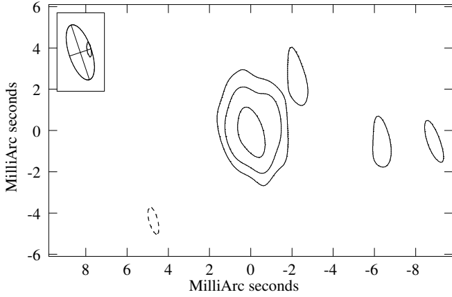
Fig. 4. VLBA 8 GHz image of IRAS 17020+4544 on 2012 Feb. 8, with contours traced at (-1, 1, 2, 4) \times the \sim 3\sigma noise level, which is 1.0 \text{ mJy beam}^{-1} . The half peak beam width is shown in the upper left corner and it is 2.8 \text{ mas} \times 1.1 \text{ mas} in PA 18^\circ .
