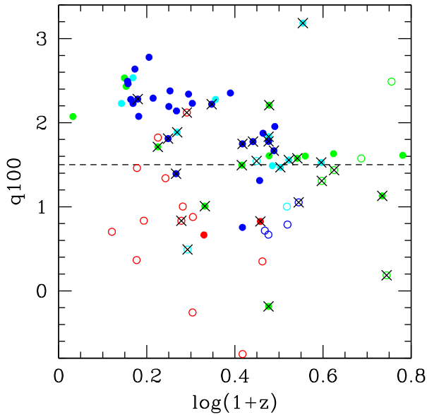
Figure 10. The q_{100} = \log(S_{100\ \mu\text{m}}/S_{1.4\ \text{GHz}}) as a function of redshift for the 5.5 GHz radio-selected sample with full IRAC detection. Symbols are the same as in Fig. 8, except that open symbols are used for sources that have only an upper limit at 100 \mu\text{m} .
