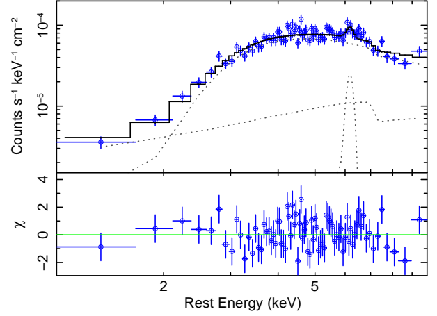
Figure 7. Upper panel: The model composed of an intrinsically absorbed power-law plus a continuum reflection component and one narrow emission line ( tbabs*(ztbabs*zpowerlw+pe\text{trav}+zgauss) , model 3 in Table 3) is plotted over the XRT spectrum of MCG+11-11-032. Lower panel: Relevant residuals plotted in terms of sigmas.
