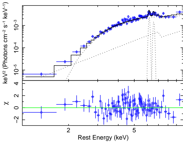
Figure 9. Upper panel: the model, which includes an intrinsically absorbed power-law plus a continuum reflection component and two emission narrow lines ( tbabs*(ztbabs*zpowerlw+pe xrav+zgauss+zgauss) ), model 4 in Table 3), is plotted over the spectrum of MCG+11-11-032. Note that this plot was obtained by creating fluxed spectrum against a simple \Gamma = 2 power-law and then overlaying the best fit model. Lower panel: relevant residuals, plotted in terms of sigmas.
