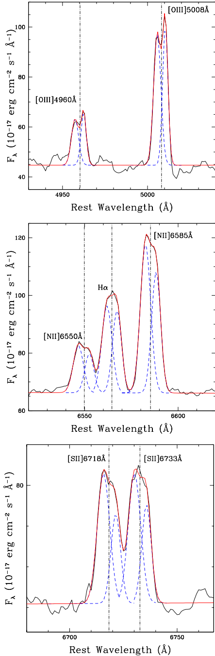
Figure 2. MCG+11-11-032 rest-frame spectrum around the [OIII] (top panel), H \alpha + [NII] (middle panel) and [SII] (bottom panel) regions. Wavelengths are in vacuum. Red solid lines represent the total fit, while blue dashed lines are the gaussian components. Black dot-dashed vertical lines mark the position of the line at the systemic velocity of the host galaxy.
