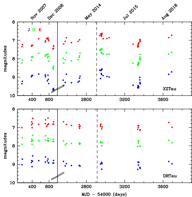
Fig. 1. Near-infrared ( JHK bands) lightcurves of XZ Tau ( top ) and DR Tau ( bottom ) based on observations taken within the EXORCISM programme around the date of GIANO observations, which is indicated by the vertical dashed line.
