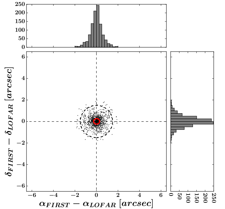
Fig. 8. Corrected positional offsets between high S/N and compact LOFAR sources and their FIRST counterparts (see text for more details). The dashed lines denote a circle with radius r = 1.5'' , which is the image pixel scale. The ellipse (red solid line) centered on the right ascension and declination mean offsets indicates the standard deviation for both directions.
